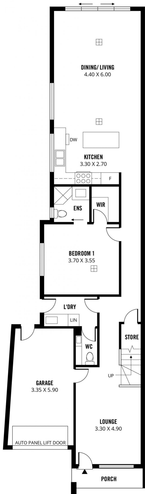
LOWER FLOOR
