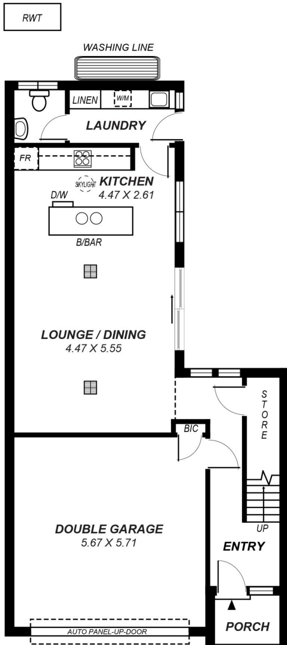
GROUND FLOOR
