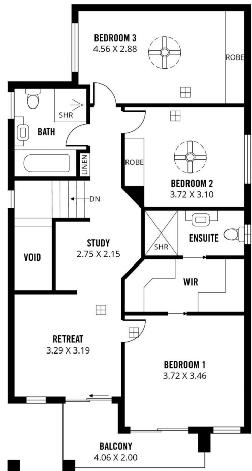
UPPER FLOOR
